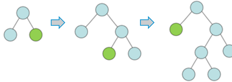
Leaf-wise growth
