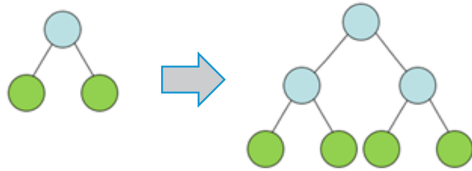
Level-wise growth
